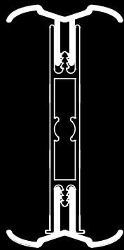
10mm I_x = 11.17\text{cm}^4 I_y = 0.41\text{cm}^4 AE10/SMART
