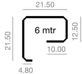
AE212IGS/3 'NEW' CASEMENT SASH
