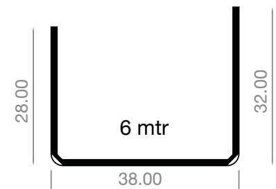
AE3238GS/HD3 TILT/TURN SASH
