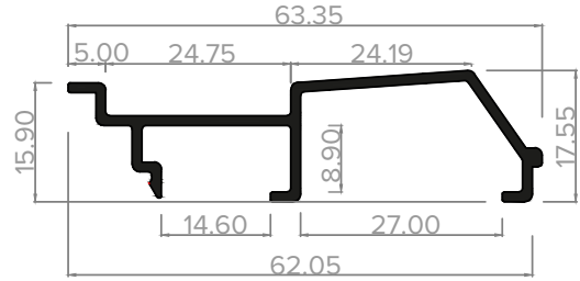
AEDMA/EURO - EWS 7512 A MEETING STYLE ADAPTOR
