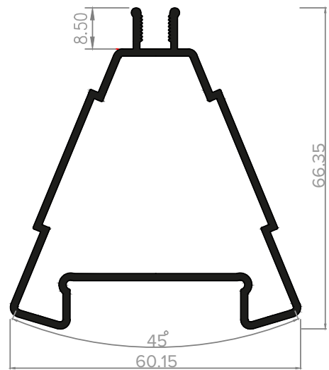
AEI35/EURO - EWS 517 A 135° BAY POST
