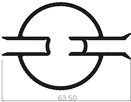
AEBPI70/EURO - EWS 7523 A 150° - 170° BAY POLE
