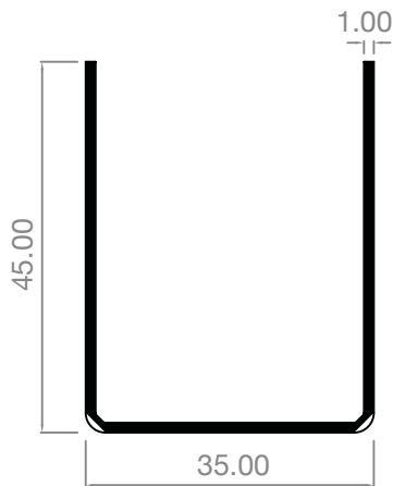
AE323GS/I9 EWS7675 I900mm lengths
