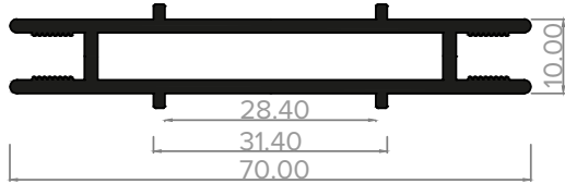
AEIO/EURO - EWS 510 A 10mm COUPLER/BUTT JOINT
