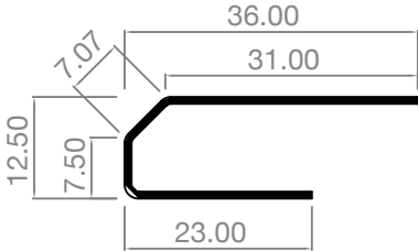
AEI337GS (EWS7604S) INT/EXT CASE SASH
