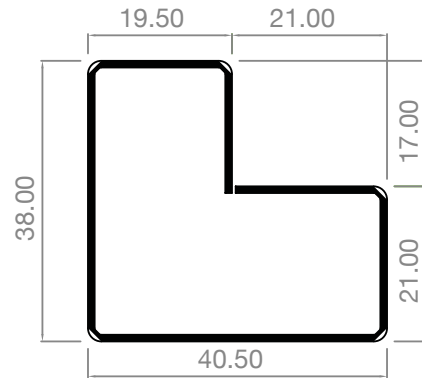
AE3841GS (EWS616S) DOOR OUTER
