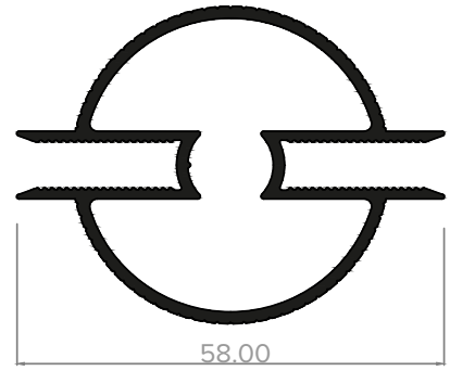
AEBPI50/EURO - EWS 523 A 120° - 150° BAY POLE
