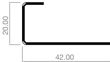
AE2042GS/3 (EWS7607S) TILT/TURN
