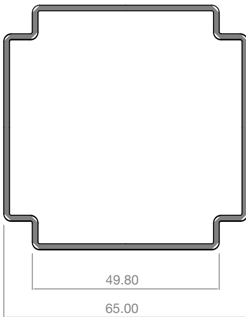
AEL6565 ALUMINIUM POST 6000mm lengths
