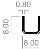
AE88GS/I9 EWS7676S I900mm lengths
