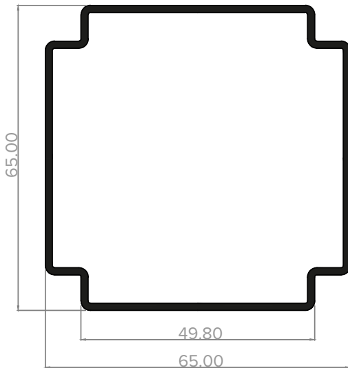
AEL 6565 - EWS 520 A 65mm SQUARE CORNER POST
