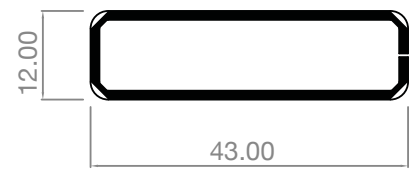
AE4112GS (EWS601S) C. OUTER/TRANSOM T & Z
