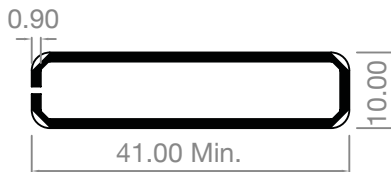
AE4210GS/IW slim trans/mullion T/Z 69mm 52mm slim outer 62mm int outer
