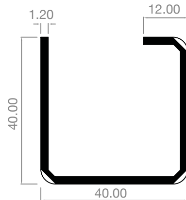
AE4040GS/IW Door Sash, T & Z, Midrail
