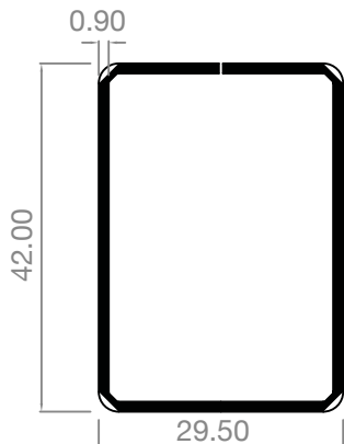
AE4230GS/IW 72mm univ. outer comp door outer
