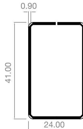
AE4224GS 82mm T & Z mullion
