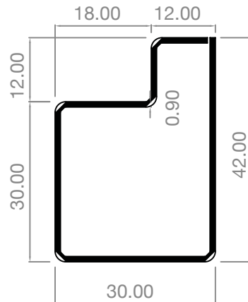
AE4230GS/EDG 72mm univ. outer comp door outer
