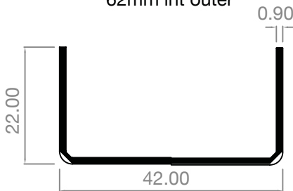
AE4020GS 70mm T/Turn sash
