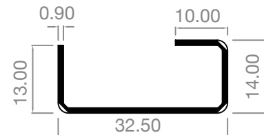
AE223GS/ORIOS casement Z sash
