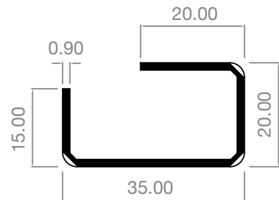
AE3520GS/IW 75mm T sash
