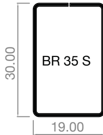
AE/BR35S T & Z casement & bevel/ovolo
