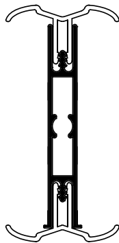
10mm I_x = 11.17\text{cm}^4 I_y = 0.41\text{cm}^4 AE10/SMART
