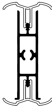
16mm I_x = 11.35\text{cm}^4 I_y = 1.26\text{cm}^4 AE16/SMART
