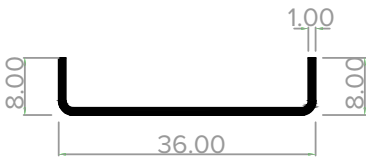
AE368GS 55mm OUTER
