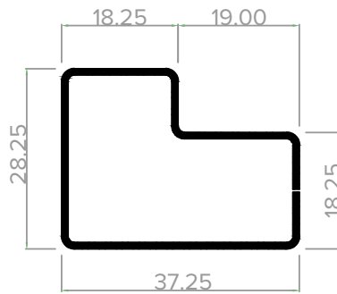
AE2837GS KEEP RELIEF
