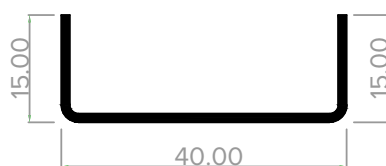
AE4015GS CILL
