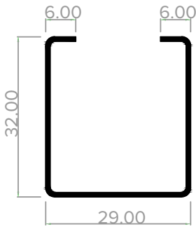
AE2932GS
