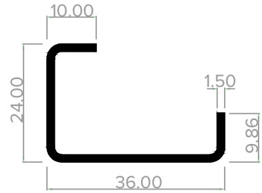
AE3624GS 82mm TILT & TURN
